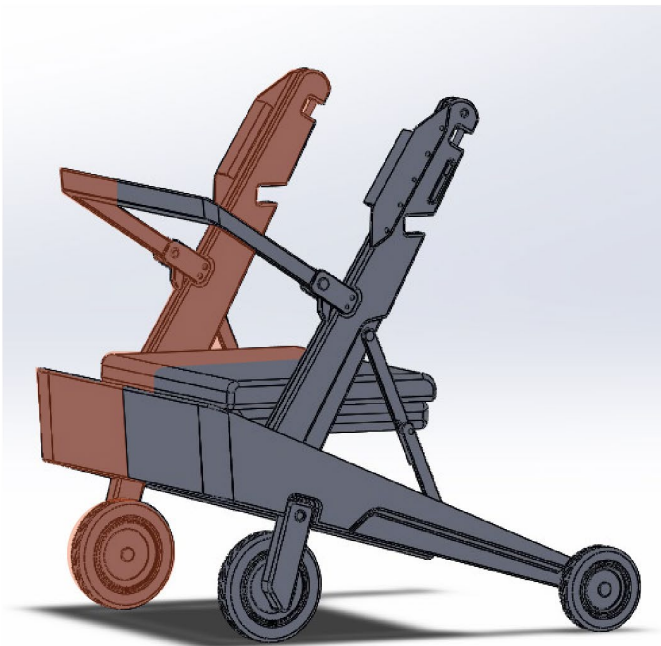
Tray Development
